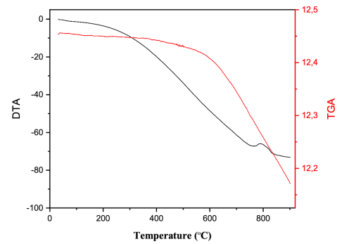
Figure 4. Thermalgravimetric Pattern Of Graphite
