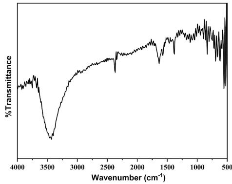
Figure 2. FT-IR Spectrum Of Graphite
