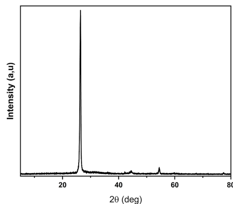
Figure 1. X-ray Powder Diffraction Patterns of Graphite
